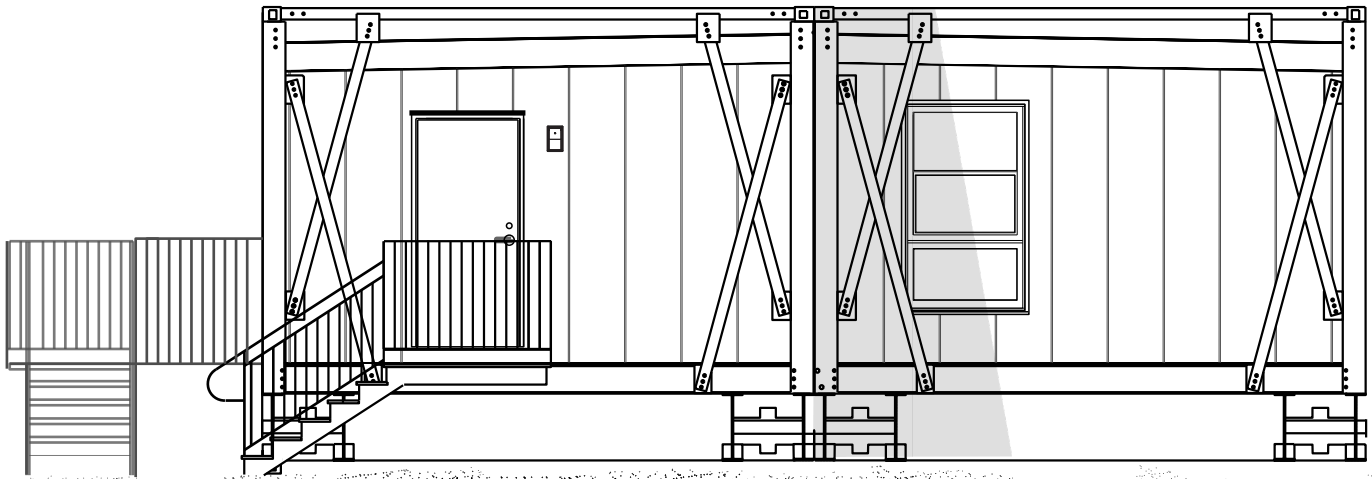
REAR ELEVATION
