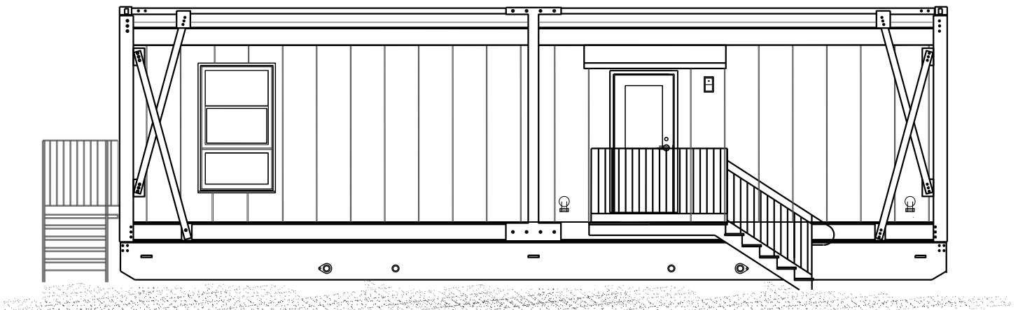
ENTRANCE ELEVATION
